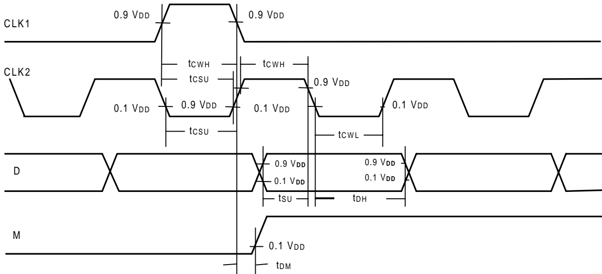
Figure 3. Sending Data to Segment Driver LSI NT3882A
