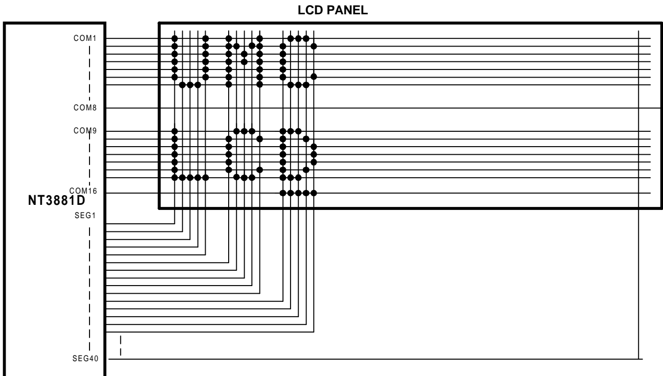
(c) 5 X 8 Font - 8 character X 2 lines (1/16 duty cycle, 1/5 bias)
